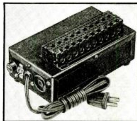
Fig. B. Here is illustrated a complete 110-V. D.C. to 110-V. A.C. polarity changer converter with an output rating of 250 W. (Electronic Labs. model 833).
